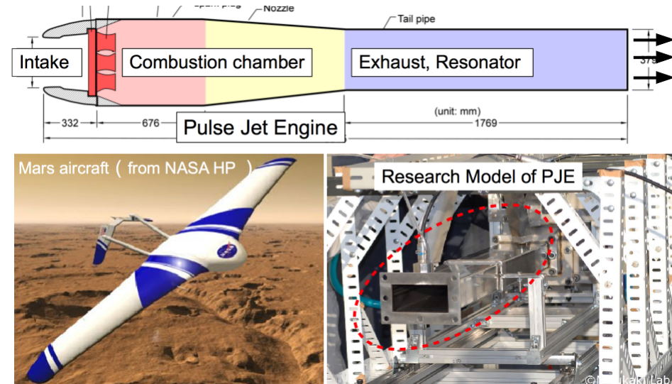
Fig. 2 Pulse detonation engine for Mars probing.
