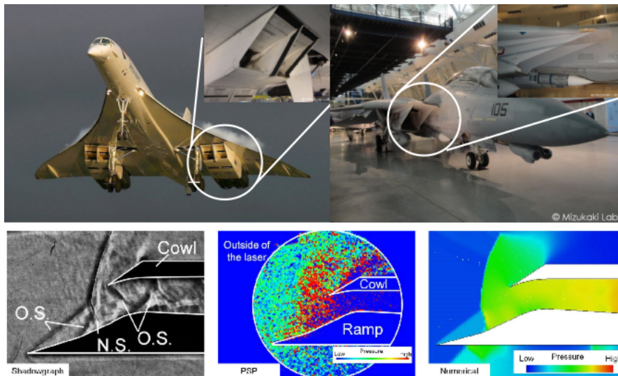
Fig. 1 Shock waves instability around supersonic inlet.
